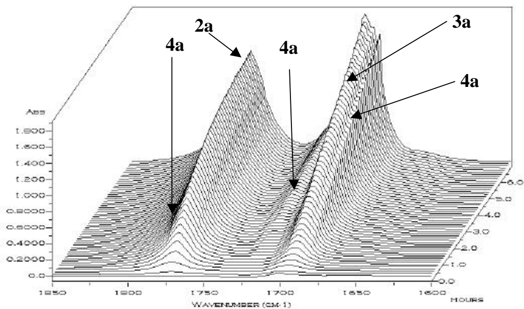
Figure 1. In situ IR spectra of the cyclo-oligomerization of 31.1 mmol n-BuNCO ( 1a ) in the presence of 4.0 mmol PBU 3 ( 5 ) at 20°C.
